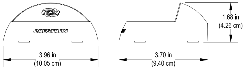
CEN-IPOD-DS Dimensions
